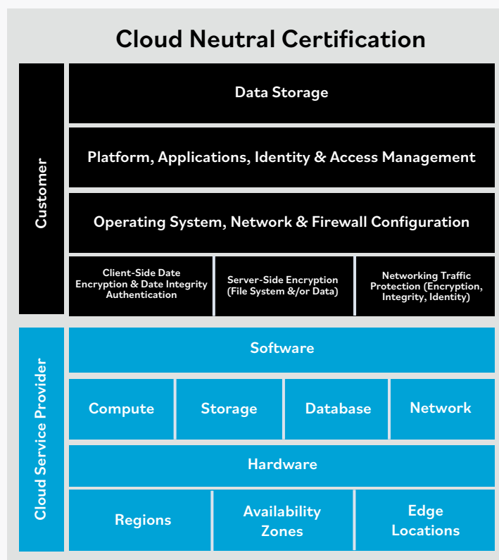
Figure 1: The Shared Responsibility Model
